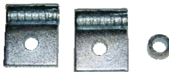
Part # 14-6B 3 Piece side clamp
