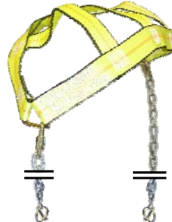
Part # 38-6 Holmes Basket Straps WLL: 1,665 lbs
