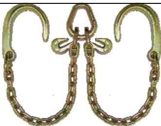
V Chain with 8" J hooks (and Grab hooks at pear link)
